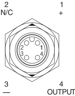
4 Pin Polarized M12 Connector (Male)
