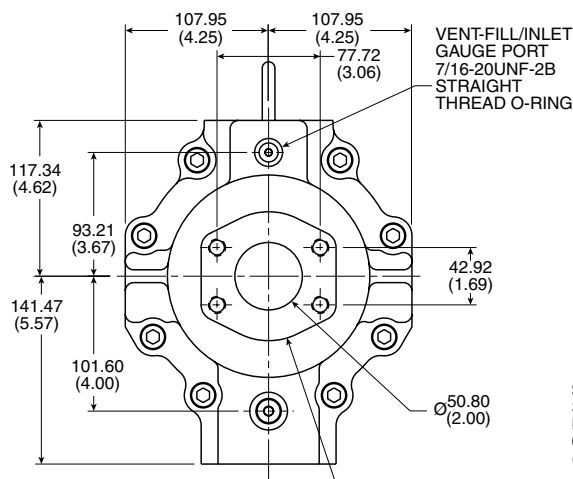
REAR INLET PORT (INLET PORT OPTION "OMIT") SEE CHART FOR PORT SIZE
