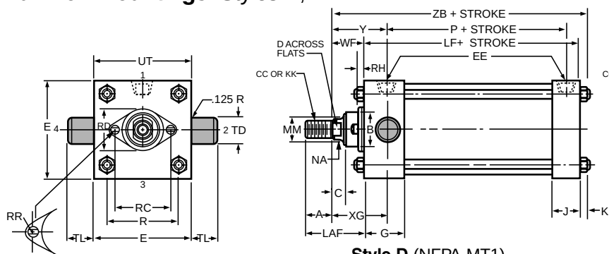
Style D (NFPA MT1)
