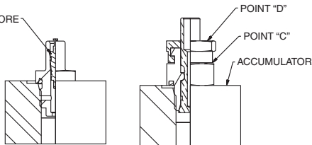
FIGURE 8A 3000 PSI VALVES
