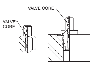
FIGURE 8A 3000 PSI VALVES
