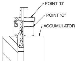
FIGURE 9 5000 PSI VALVES
